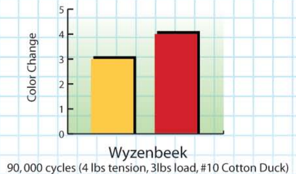
ASTM-D4157 Abrasion Color Change: Wear-Defense™ vs. No Wear-Defense™
