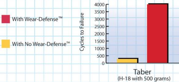
ASTM-D3884 Abrasion Testing: Wear-Defense™ vs. No Wear-Defense™
